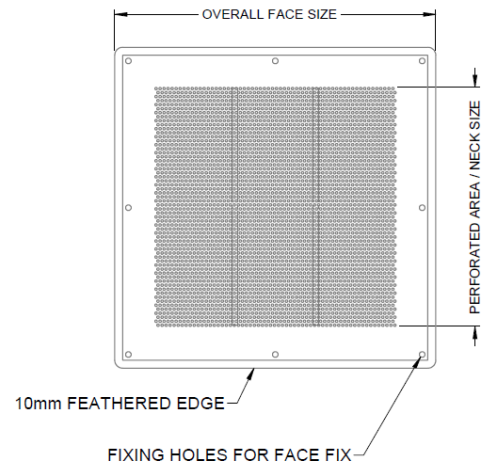
MAXIMUM SECURITY PERFORATED AIR GRILLE SE-MSP-F (FACE FIX)
