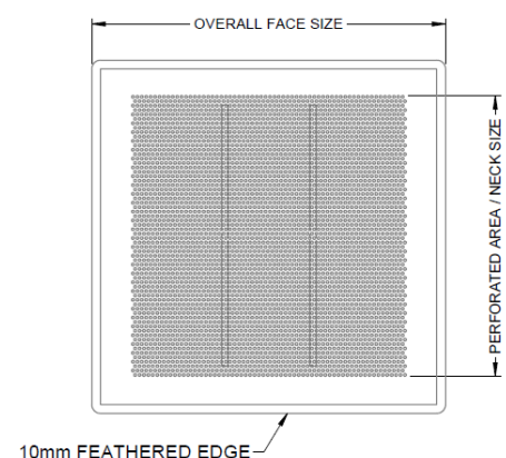
MAXIMUM SECURITY PERFORATED AIR GRILLE SE-MSP-R (REAR FIX)
